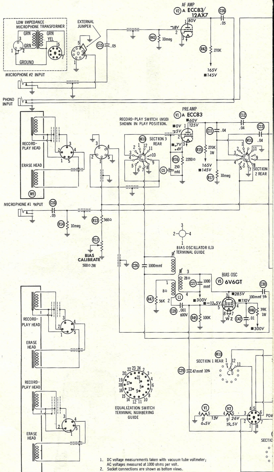
DUAL RECORD-PLAY & ERASE HEAD ASSEMBLY USED FOR STEREO OPERATION.
